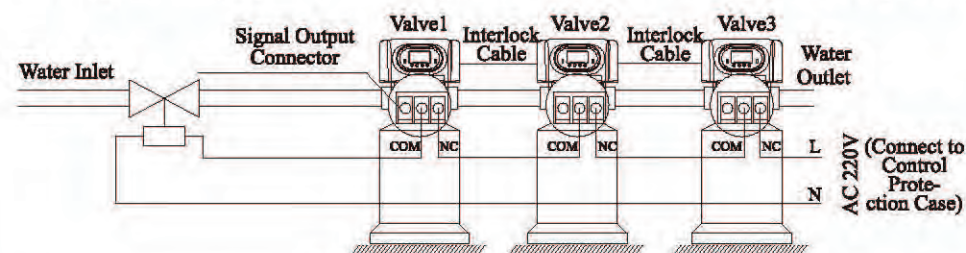
Figure 10 Wiring of Solenoid Vale in Inlet
