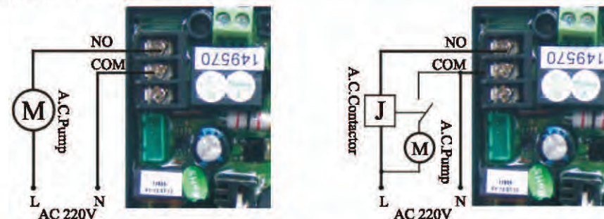
Figure13 Wiring of Booster Pump on Inlet Figure 14 Wiring of Booster Pump on Inlet
