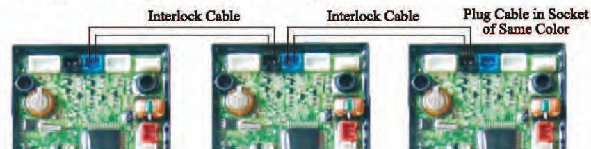
Figure15 Interlock Connect
