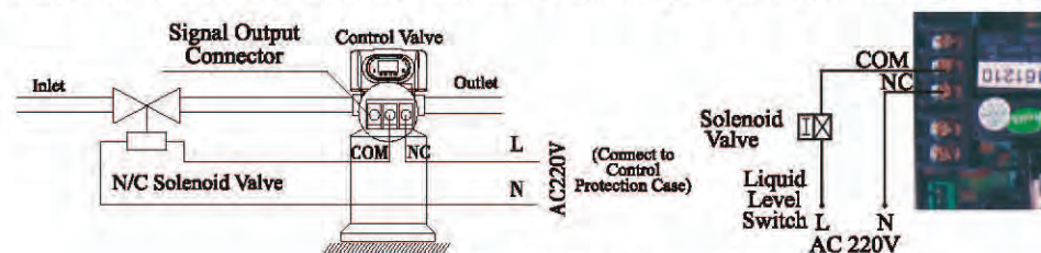
Figure 9 Wiring of Solenoid Valve on Inlet
