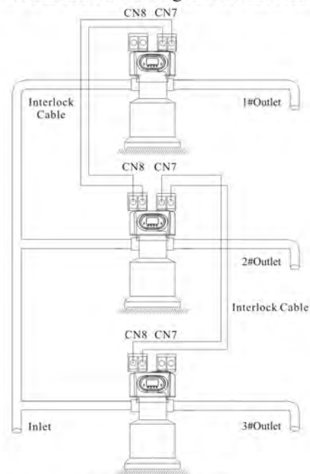
Figure 3-12 Interlock System
