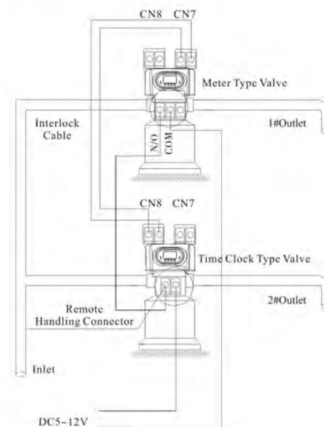
Figure 3-13 Series System
