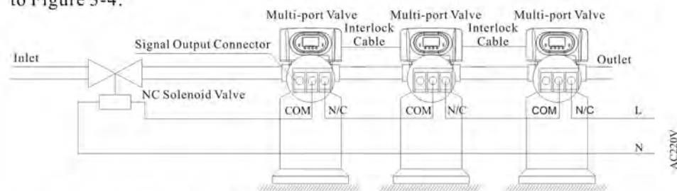
Figure 3-4 Wiring of Solenoid Valve on Inlet
