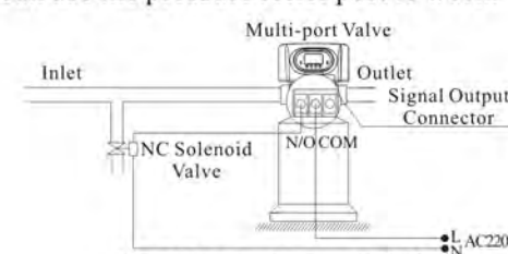
Figure 3-3 Wiring of Pressure Relief Port
