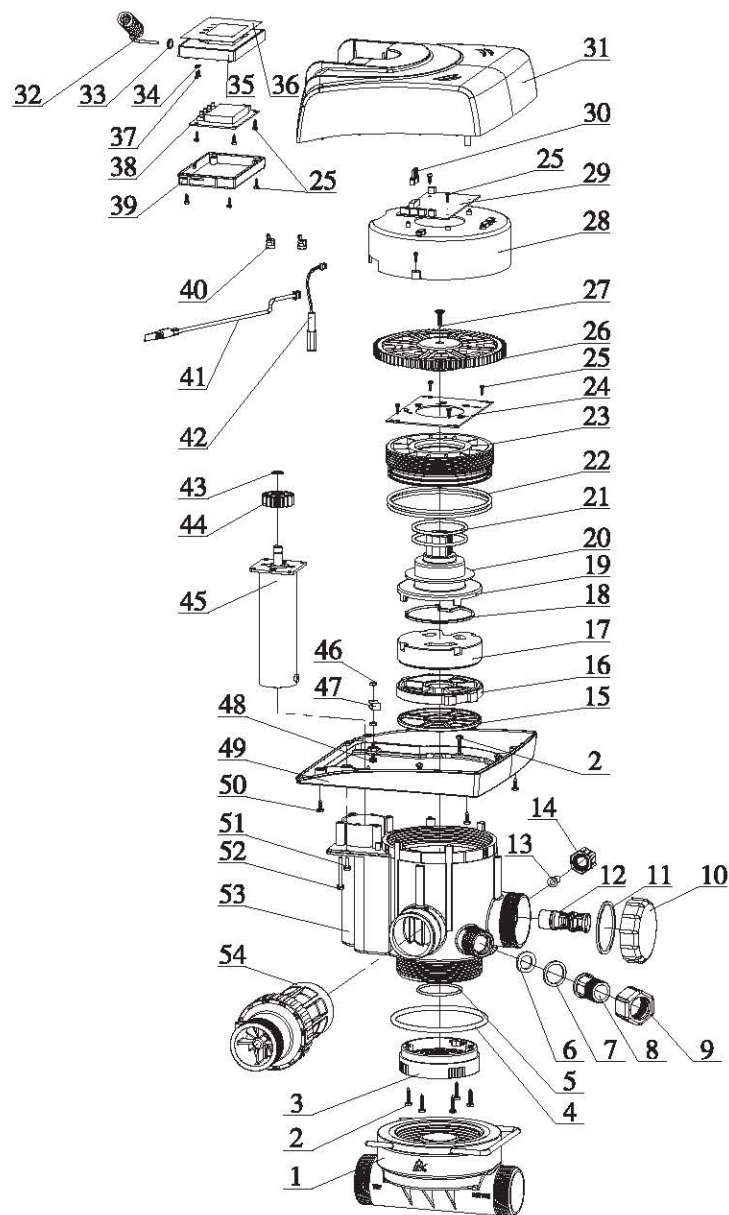
F74B3 (63510B) Structure Chart:
