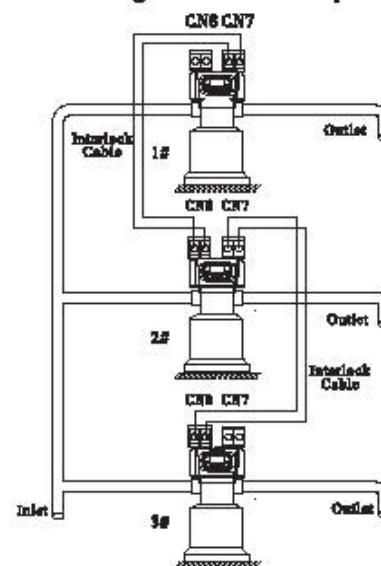
Figure 3-12 Interlock system
