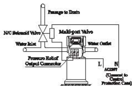
Figure 3-10 Wiring of Pressure Relief Output
