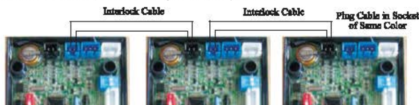
Figure 3-9 Network System Wiring with Interlock Cable
