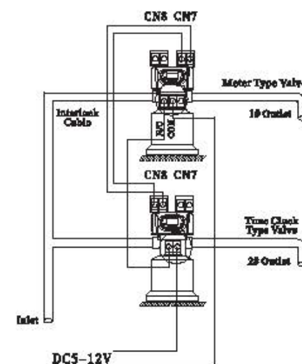
Figure 3-13 Series system
