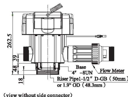
Structure Chart of F74B3 ( 63610B )
