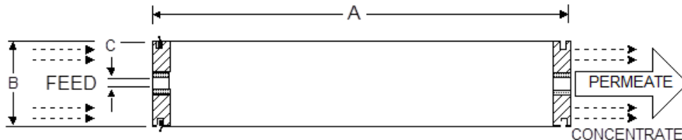
Element Details**
