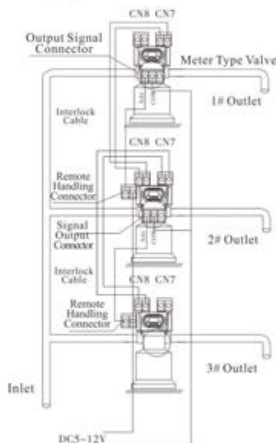
Figure 3-13 Series system
