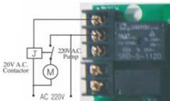
Figure 3-8 Wiring of Booster Pump on Inlet
