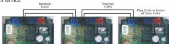
Figure 3-9 Network System Wiring with Interlock Cable
