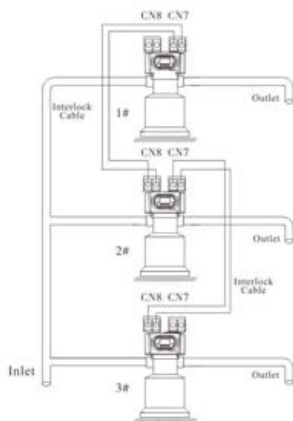
Figure 3-12 Interlock system
