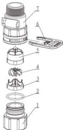
5447018 Flow Meter
