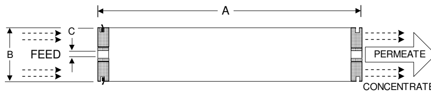
Element Details**
