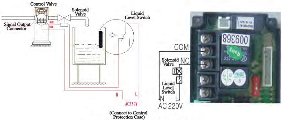
Figure3-2 Wiring of Outlet Solenoid Valve
