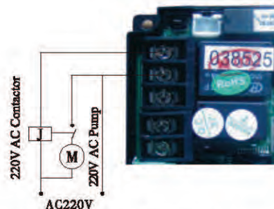
Figure 3-8 Wiring of Booster Pump on Inlet Figure 3-9 Wiring of Booster Pump on Inlet
