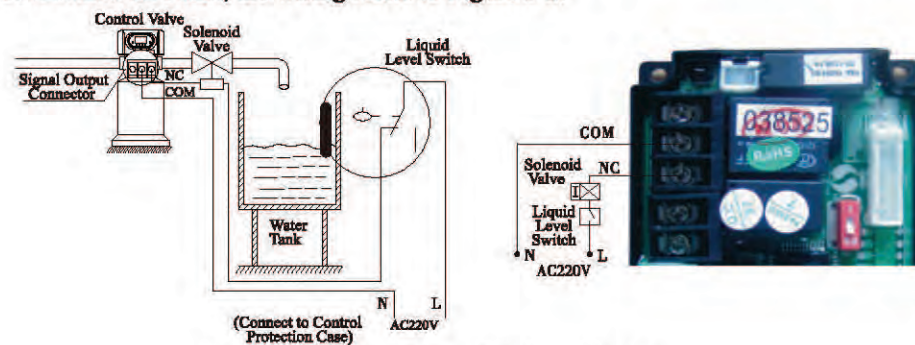
Figure 3-2 Wiring of Solenoid Valve on Outlet
