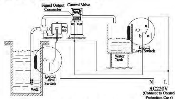
Figure 3-6 Wiring of Liquid Level Controller Controls 220V Inlet Pump
