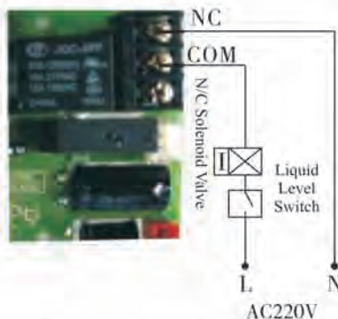
Figure 3-1 Wiring of Solenoid Valve on Outlet
