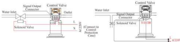
Figure 3-2 Wiring of Solenoid Valve on Inlet
